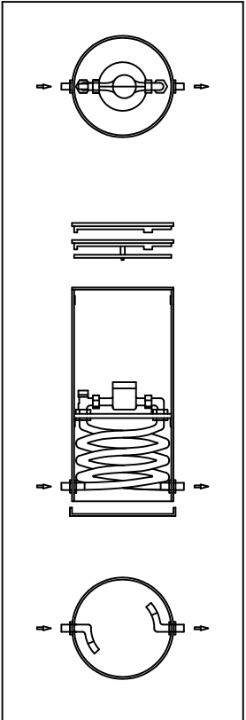
MUELLER/McCULLOUGH® THERMAL-COIL® METER BOX
