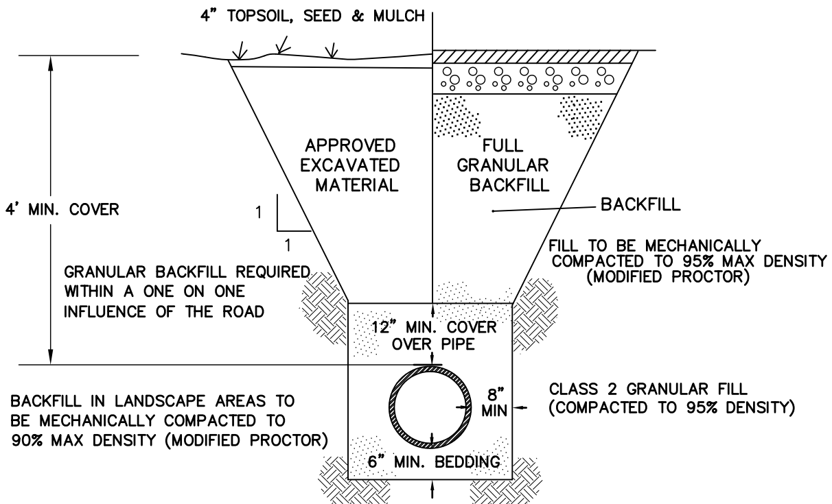
TRENCH DETAIL NO SCALE
