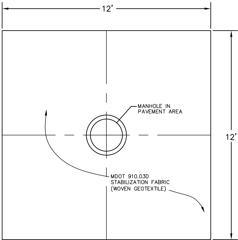
FABRIC & BITUMINOUS COLLAR DETAIL NO SCALE
